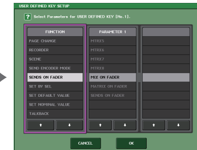
Janela USER DEFINED KEY SETUP
